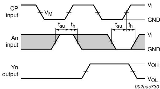
Figure 7. Data set-up and hold times, An input to LE input
